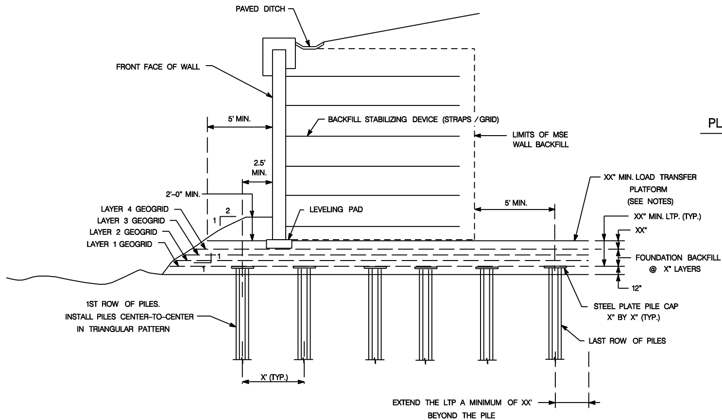
SECTION ALONG WALL
