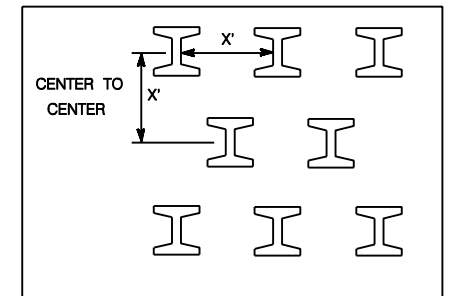
PILES CENTER-TO-CENTER IN TRIANGULAR PATTERN
